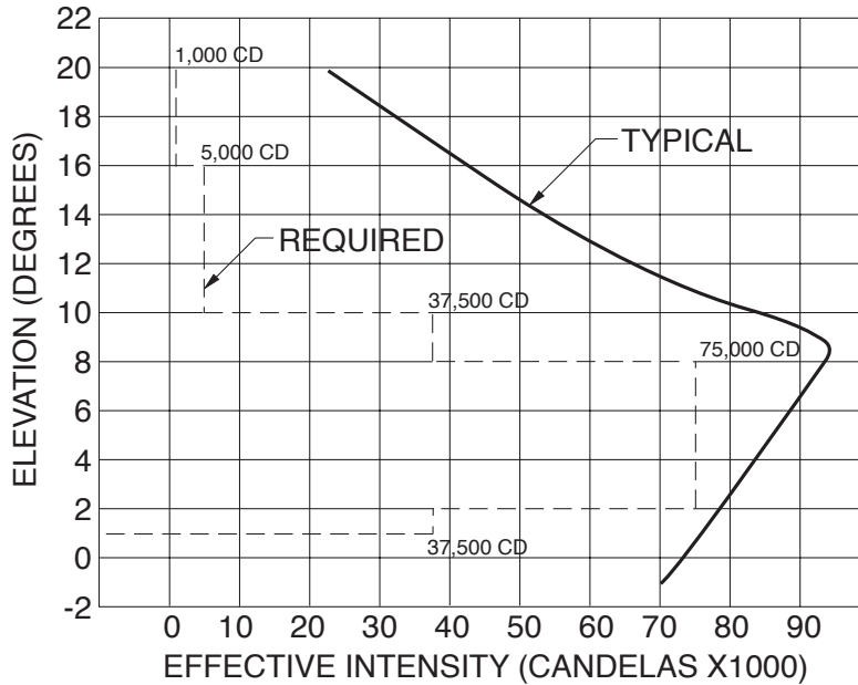
ELEVATION vs EFFECTIVE INTENSITY L-802A/S, 1000W, 2 LENS BEACON, WHITE LENS
